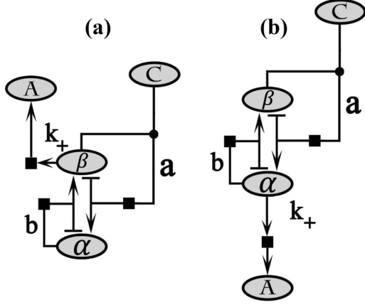
FIG. 5. Molecule C is given by the cascade. Its levels stay unchanged while it interacts with molecule \beta to produce molecule \alpha . In (a), we see molecule \beta drives molecule A . Thus, C acts as a repressor for A . If we move A to be driven by \alpha , then C works as an activator for A . Notice that creation of A is not accompanied by an annihilation of \alpha or \beta , as is commonly seen in the Michaelis-Menten process. Adding an additional action line to include the missing annihilation would only create, in the mathematical formulas, sums of the form k_+ + b . Since b \rightarrow \infty and k_+ is finite, the effect of an additional action line is irrelevant. Similar approaches are taken for the deterministic case in Refs. [11,28–30].
